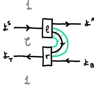
Figure 3: An optic embedded into Prof . Note how the coend condition becomes invisible to the diagrammatic calculus. Here we use \mathfrak{L}_\square and \mathfrak{L}^\square to denote the covariant and contravariant Yoneda embedding.
