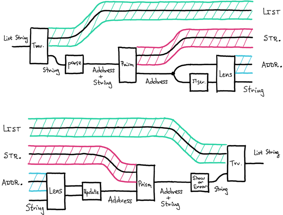
Figure 2: An example of direct composition in monoidal notation.
